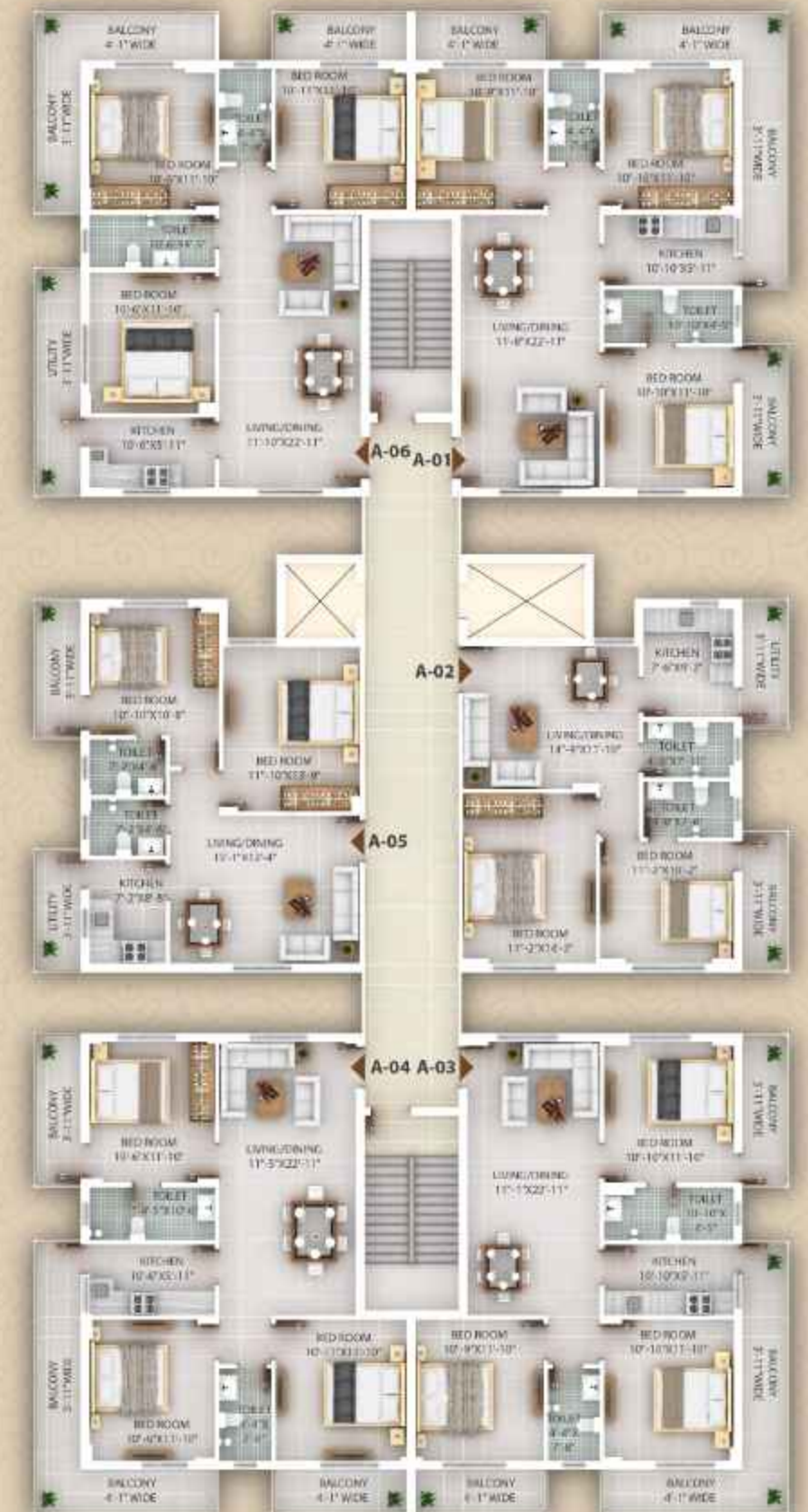
BLOCK A - 2ND TO 9TH FLOOR
